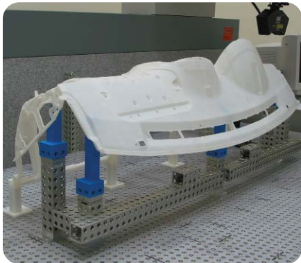
Image 1: Kia Spectra. Image 2: Design rendering of Kia Spectra dashboard. Component fit is very important to Hyundai. Image 3: The CMM scan showed the ABS Prototype was within tolerance.
